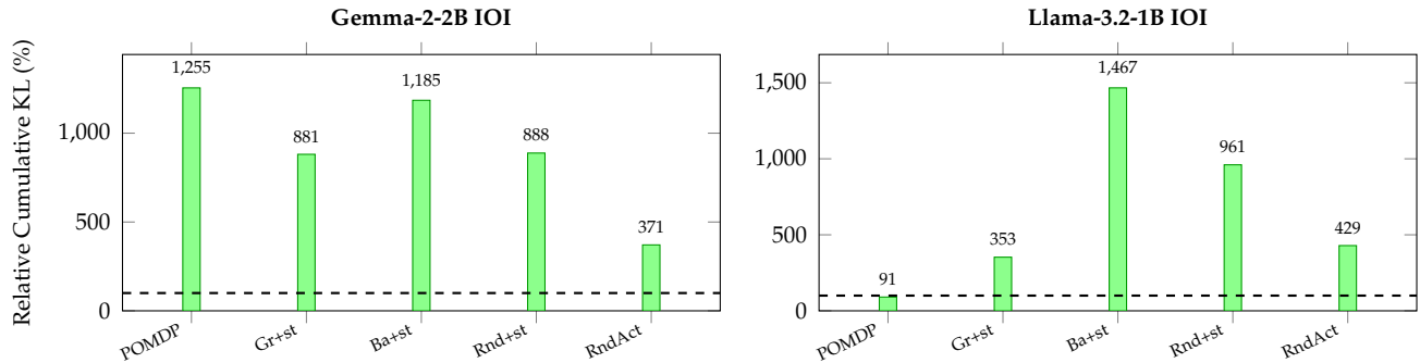
Figure 7: Oracle efficiency across IOI and multi-step tasks for Gemma-2-2B Relative Cumulative KL of the multi-action POMDP against action-matched baselines (left Gr+st, Ba+st, Rnd+st) and Llama-3.2-1B a random-action control (right RndAct), relative to the ablation oracle (100%, dashed).
