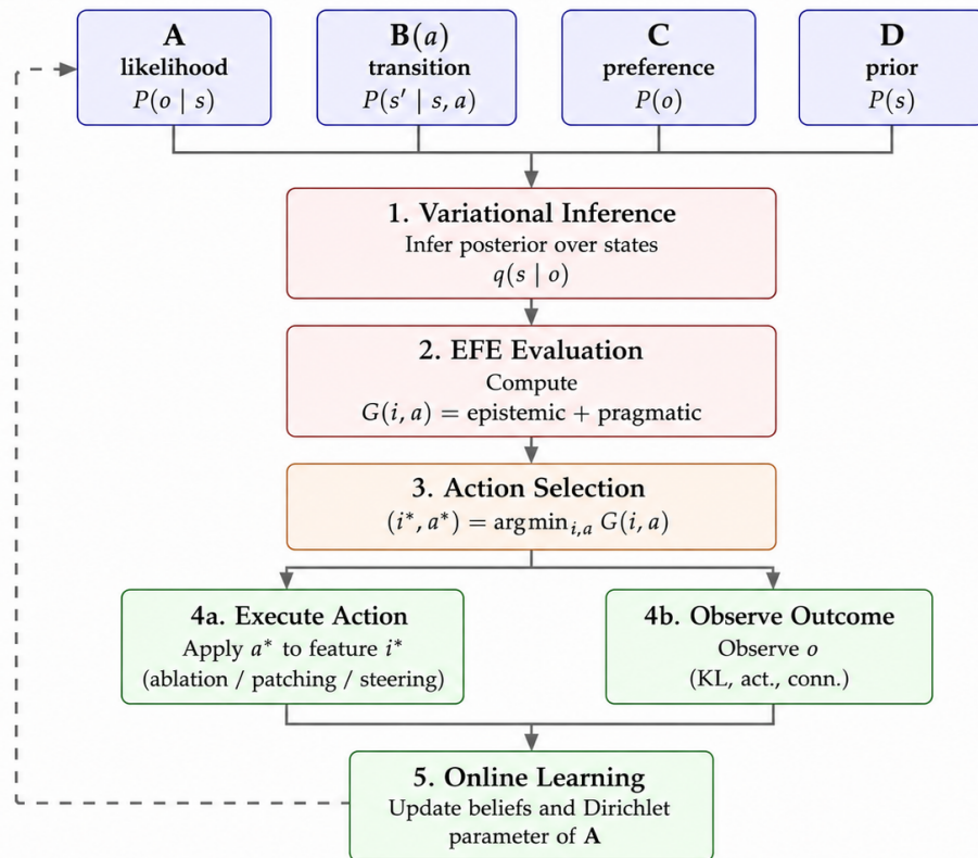
Figure 2: Active Inference POMDP agent pipeline: inference, EFE evaluation, and action selection.
