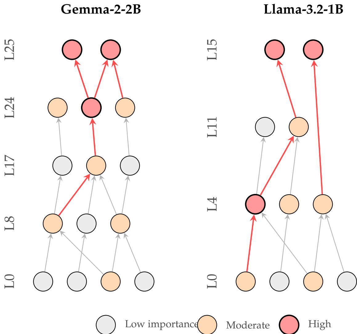
Figure 5: Simplified attribution graphs for IOI: Gemma-2-2B (left) and Llama-3.2-1B (right).
