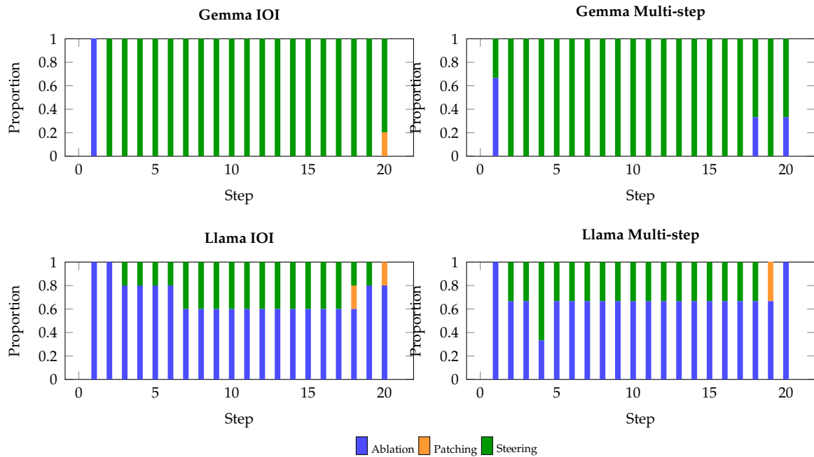
Figure 10: Action type distribution across intervention steps for Gemma-2-2B (top) and Llama-3.2-1B (bottom).
