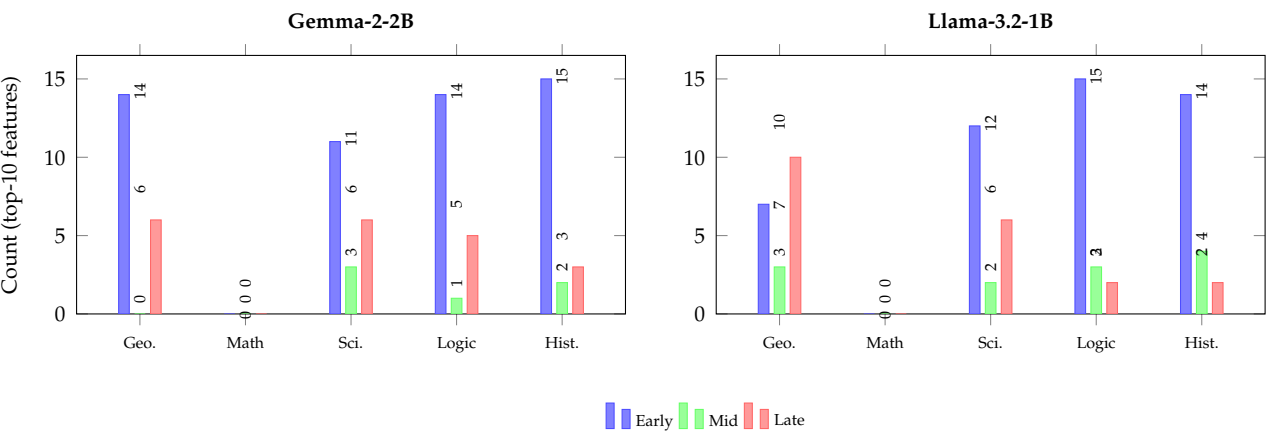
Figure 12: Layer distribution of top-10 causal features across five cognitive domains on both models.
