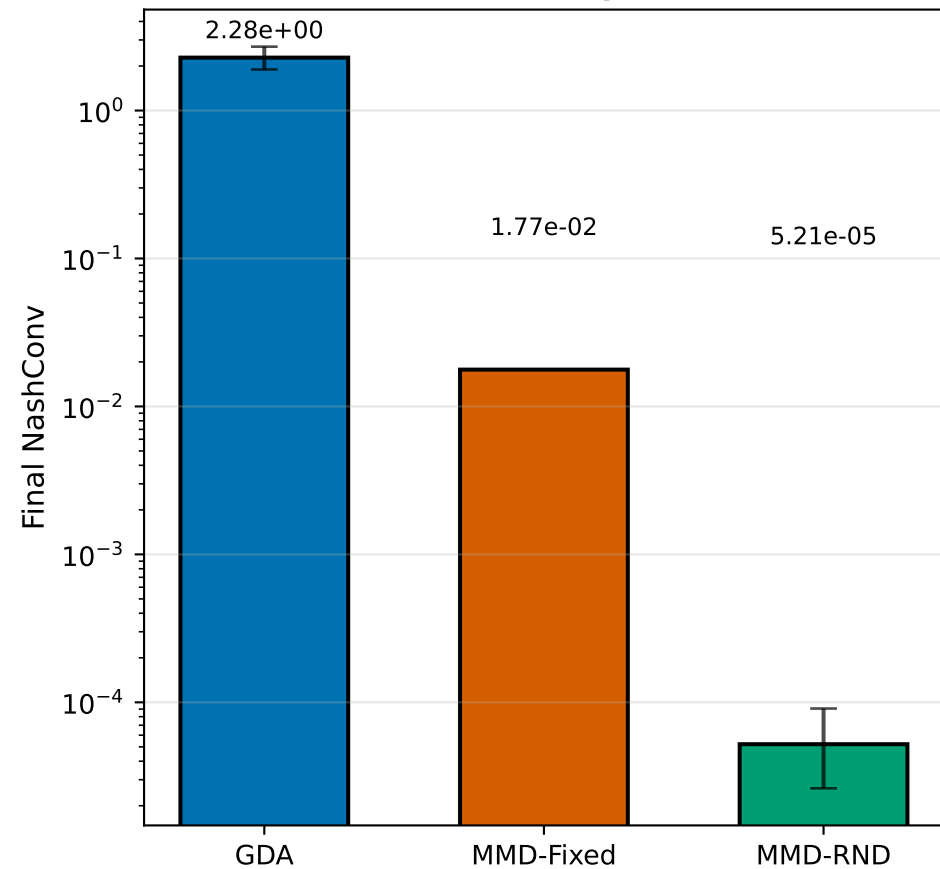
Biased Rps
