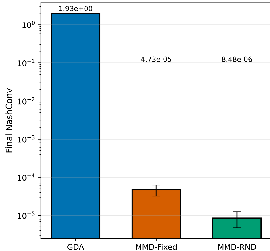
Matching Pennies
