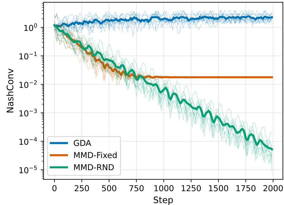
Biased Rps
