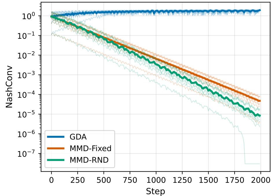
Matching Pennies
