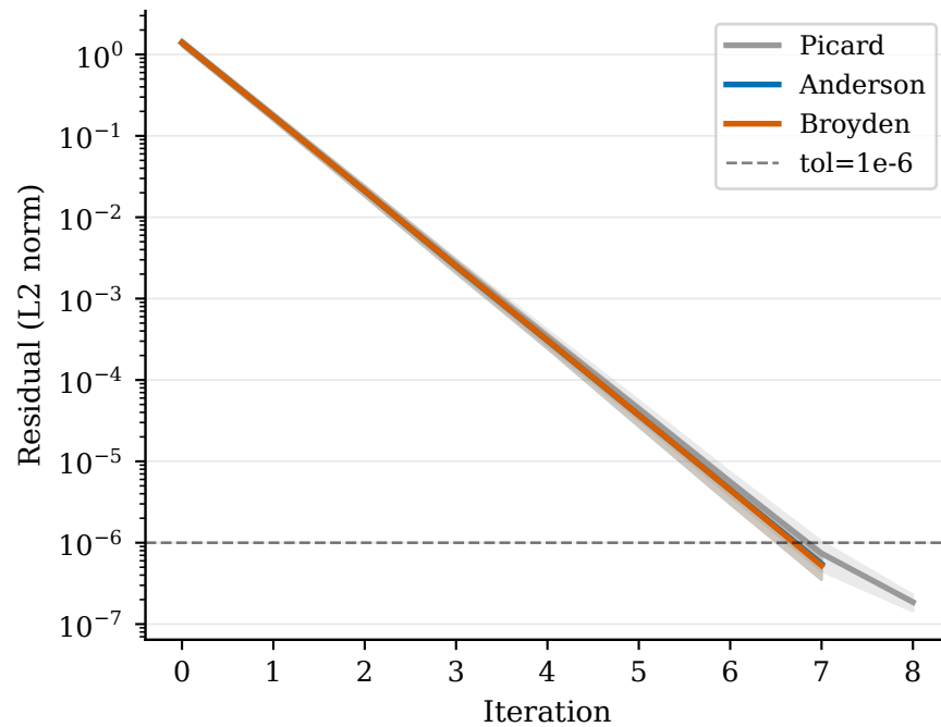
Dimension 32
