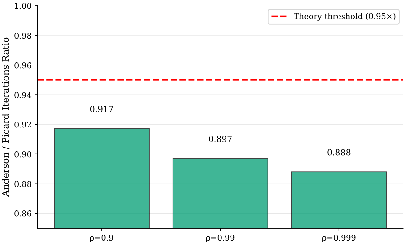
Anderson Acceleration on Tanh Contractions (dim=32)
