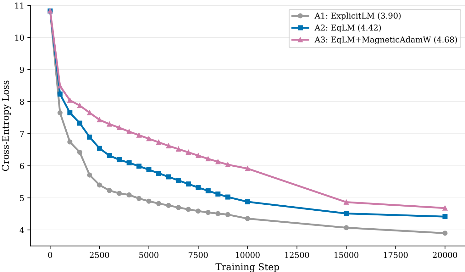
EqLM Full Run: 20k Steps, Param-Matched Arms (F13)
