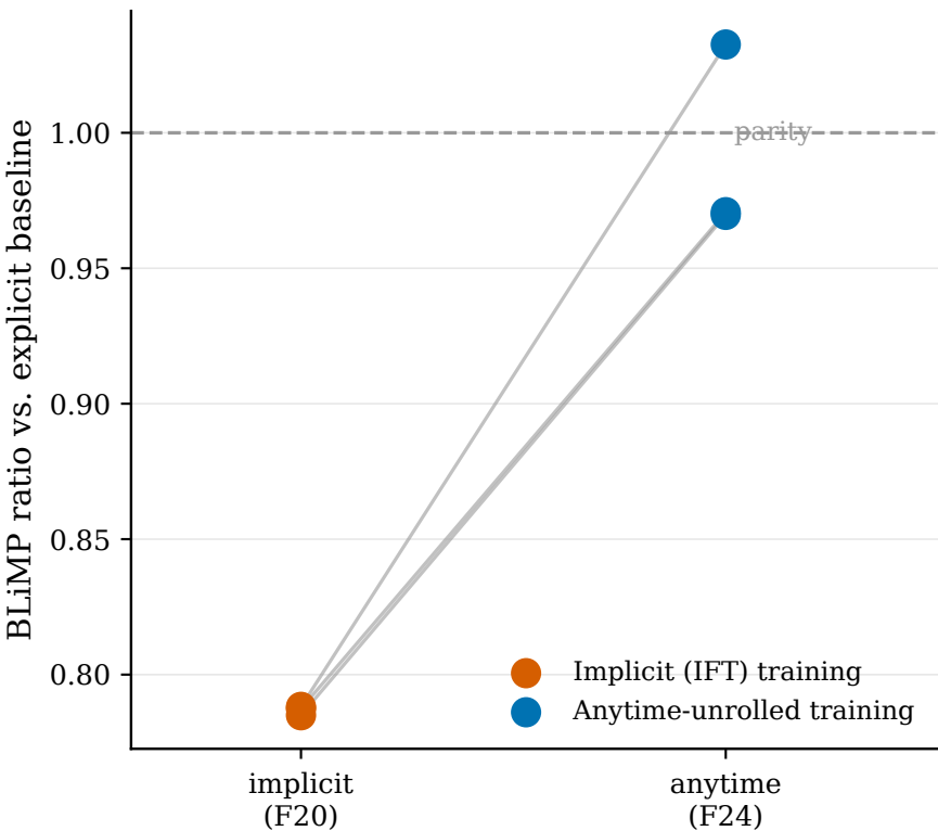
Training regime decides the width gap (121M, 3 seeds)
