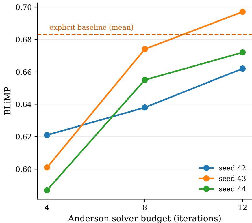
One checkpoint, three inference budgets
