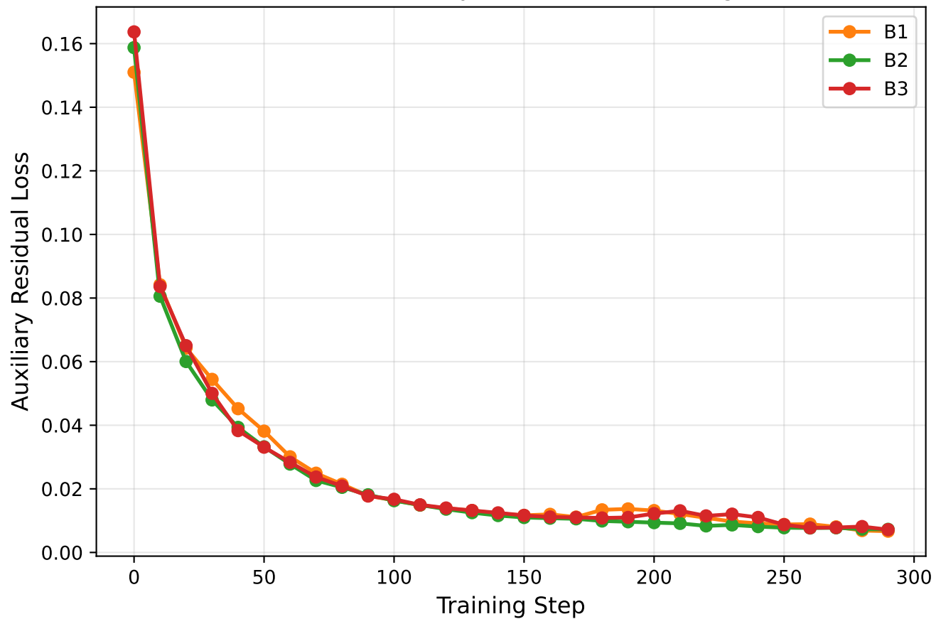
EXP08: Auxiliary Residual Over Training
