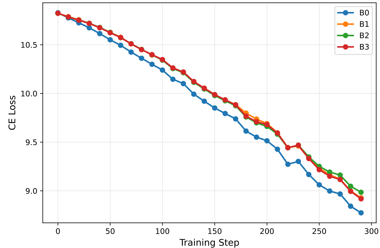
EXP08: Solver-Aware Loss — CE Loss Curves
