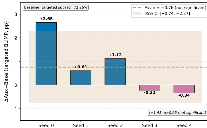
Figure 4: F3 auxiliary objective validation: per-seed performance delta (auxiliary with kāraka roles minus baseline) across 5 pre-registered seeds on the 20-paradigm targeted subset at 10M scale. The 5-seed mean delta is +0.76 pp with 95% CI [-0.74, +2.27], not significant.
