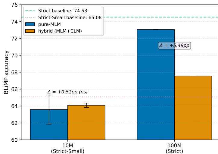
Figure 2: F1 scale-dependent objective effect: pure-MLM versus hybrid MLM+CLM performance across 10M and 100M pretraining budgets. At 10M, confidence intervals overlap; at 100M, pure-MLM achieves a 5.49 percentage point advantage.
