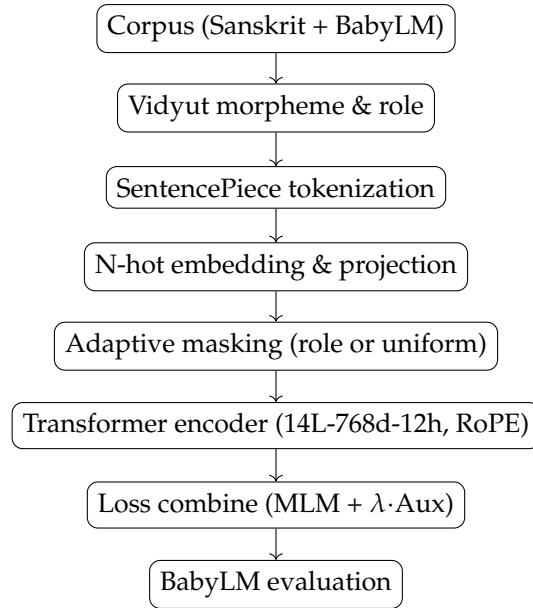
Figure 1: ELC-Prabhāsa pretraining pipeline: corpus annotation via Vidyut, N-hot morpheme embedding, adaptive masking stratified by kāraaka role, a Transformer encoder, and multi-task training combining masked language modeling with an optional auxiliary role-prediction objective that is discarded after training.
