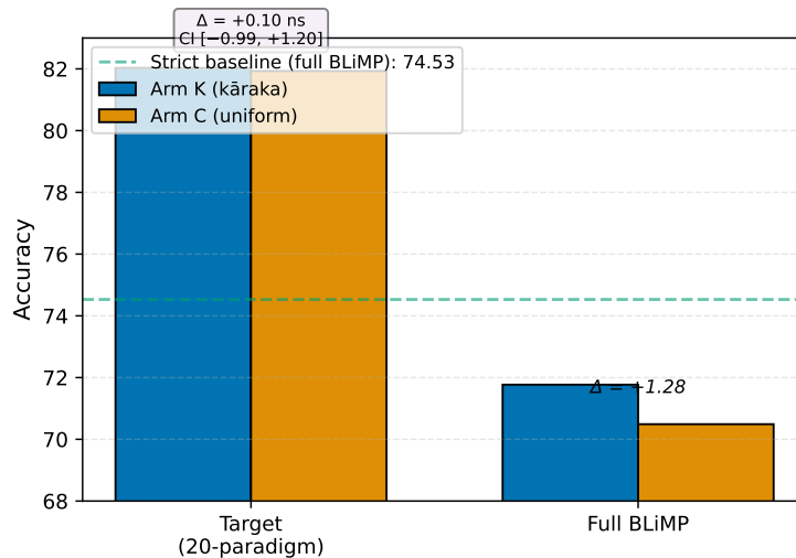
Figure 3: F2 kāraka masking causality: targeted-subset performance for Arm K (role-stratified masking) and Arm C (uniform random masking) at matched mask budget (100M scale). Paired bootstrap difference is +0.10 pp with 95% CI [-0.99, +1.20] , not significant.
