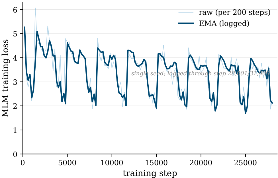
100M Strict run (prabhasa-b\_s) — MLM training loss
