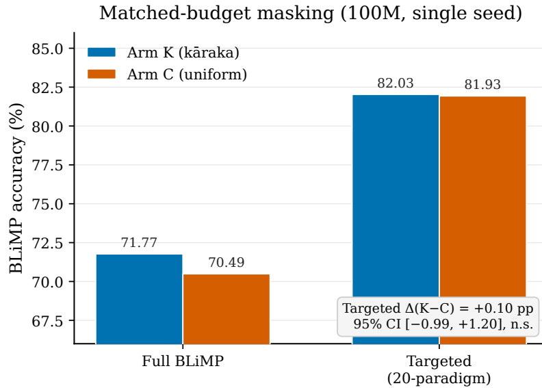
Figure 4: F2 kāraka masking causality: Arm K versus Arm C on full and targeted BLiMP (100M tokens).
