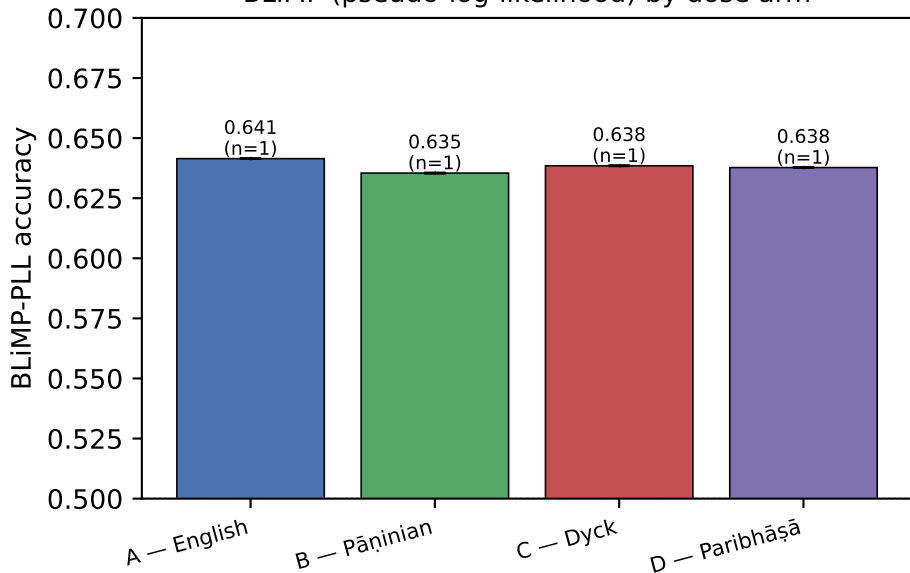
BLiMP (pseudo-log-likelihood) by dose arm
