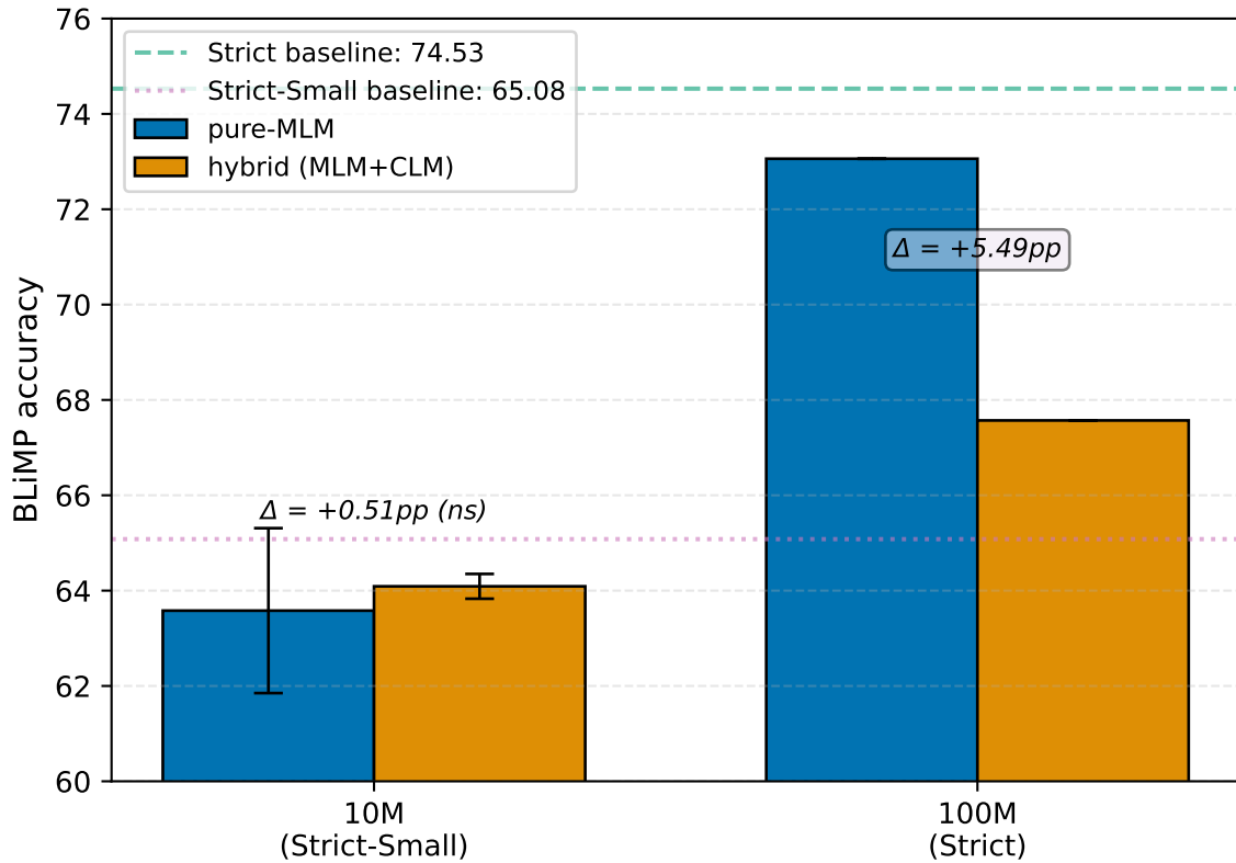
Figure 1: F1 scale-dependent objective effect: pure-MLM versus hybrid MLM+CLM performance across 10M and 100M pretraining budgets. At 10M, confidence intervals overlap; at 100M, pure-MLM achieves a 5.49 percentage point advantage.
