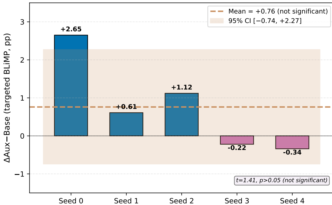
Figure 3: F3 auxiliary objective validation: per-seed performance delta (auxiliary with kāraka roles minus baseline) across 5 pre-registered seeds on the 20-paradigm targeted subset at 10M scale. The 5-seed mean delta is +0.76 pp with 95% CI [-0.74, +2.27], not significant.
