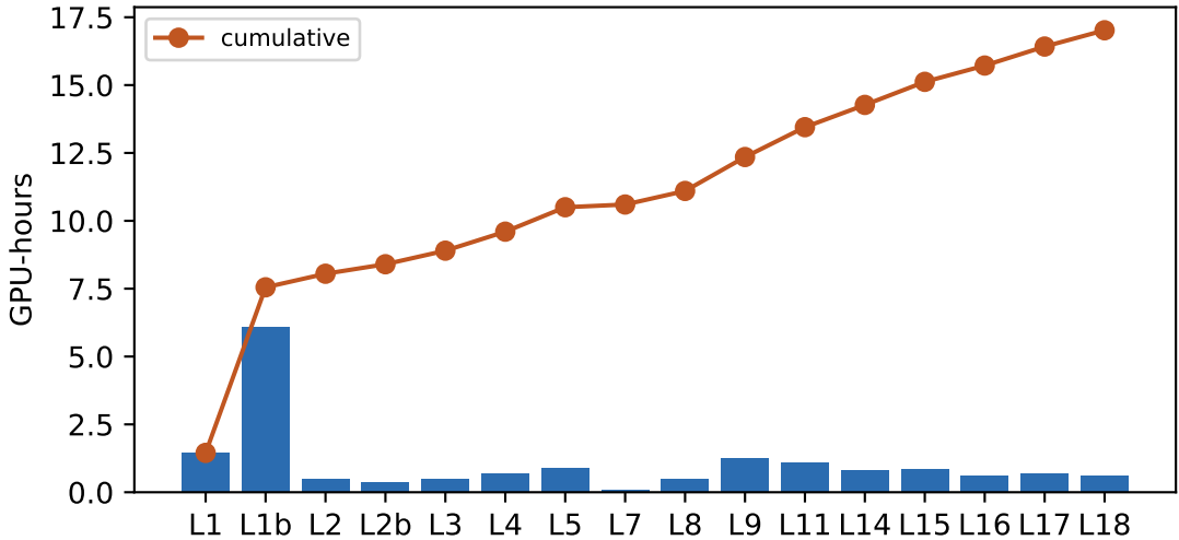
Compute ledger (total 17.0 GPU-h, one DGX Spark, guard-shared with co-resident training)
