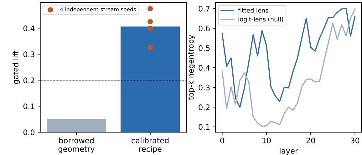
Qwen3-4B transfer: method vs geometry (confidence) | Articulation gradient: model-intrinsic
