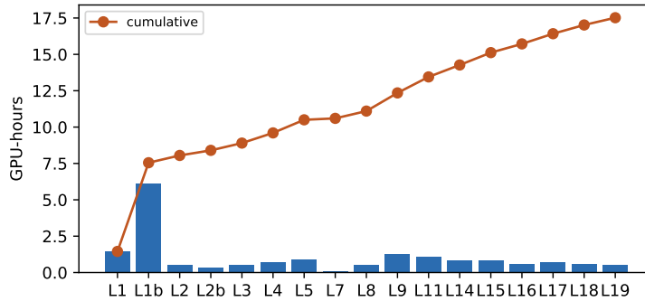
Compute ledger (total 17.5 GPU-h, one DGX Spark, guard-shared with co-resident training)
