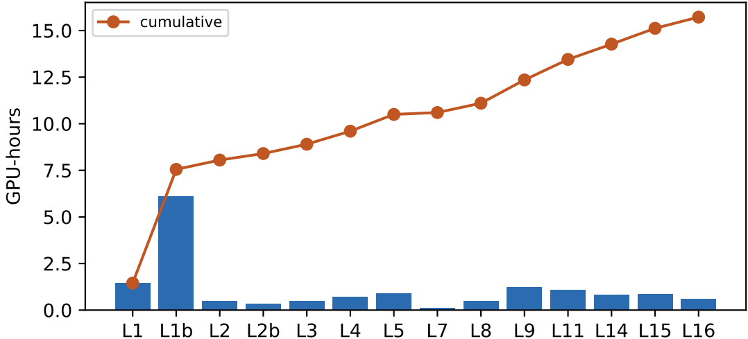
Compute ledger (total 15.7 GPU-h, one DGX Spark, guard-shared with co-resident training)
