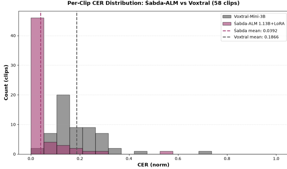
Figure 3: Per-clip CER distribution (histogram) comparing Šabda-ALM and Voxtral on 58-clip benchmark.
