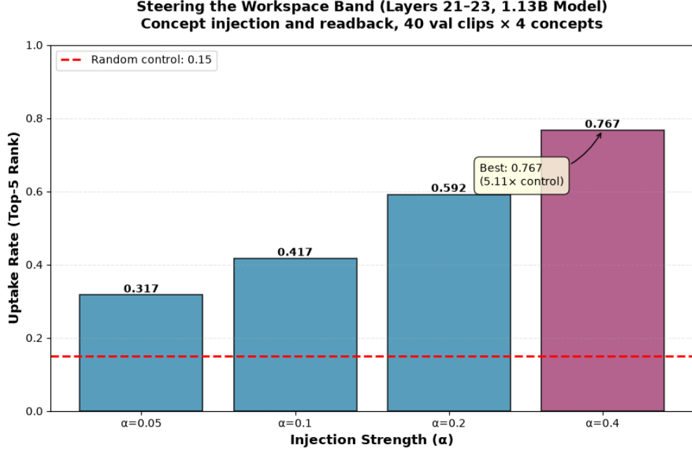
Figure 5: Steering uptake by injection strength ( \alpha ). H-SU1 satisfied: 5.11 \times control at best \alpha . H-SU3 failed: entropy collapse limits fidelity.
