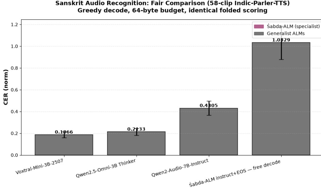
Figure 2: Leaderboard bar chart: Śabda-ALM (specialist) vs three open ALMs on fair 58-clip benchmark. Error bars are estimated CIs.
