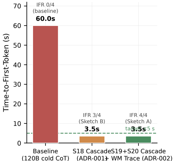
A Time-to-First-Token
