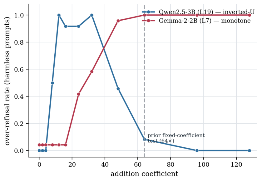
Figure 8: Single-direction addition is sufficient in both families once the coefficient is calibrated, with Qwen peaking near 12–32 before collapsing and Gemma saturating near 64.
