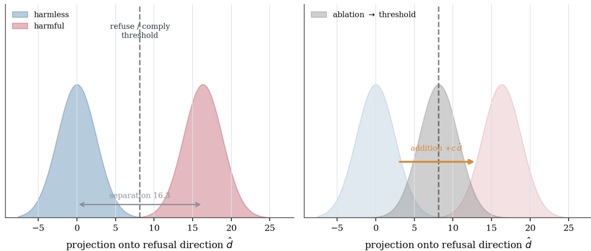
Figure 3: Harmful and harmless activations separate along the refusal direction with a measured gap of 16.3 on Gemma-2-2B (left), which ablation collapses to the threshold and addition shifts across (right).
