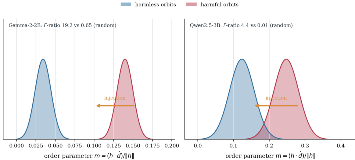
Figure 9: Distributions of the order parameter for harmful and harmless paraphrase orbits, with injection pulling the harmful band toward the harmless one in both models.
