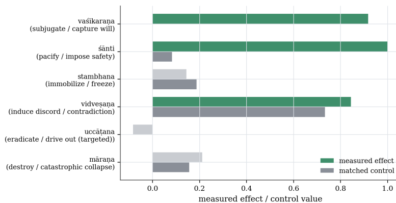
Figure 11: Three ṣaṭkarma acts control-separate from their matched controls under the naive test on Gemma-2-2B.
