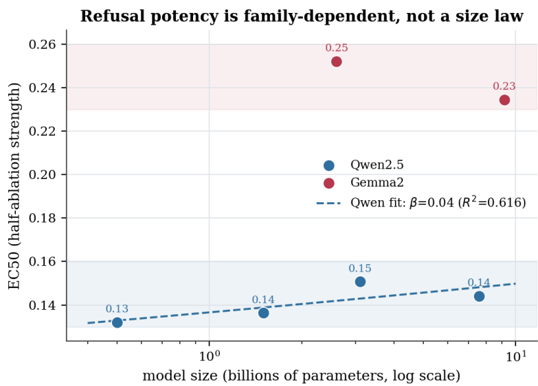
Figure 4: Refusal EC50 is family-dependent rather than a size-scaling law, with the two families separating cleanly and little within-family size dependence.
