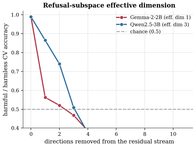
Figure 6: Removing one direction collapses harmful/harmless separability to chance for Gemma (dimension one) but not Qwen (dimension three) at their extraction layers.
