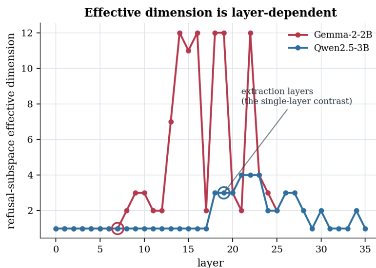
Figure 13: The refusal-subspace effective dimension varies strongly across layers, so the single-layer per-model ordering (Gemma = 1, Qwen = 3) is not representative.
