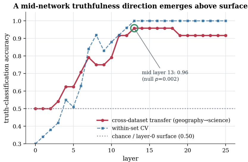
Figure 11: A mid-network truthfulness direction transfers across topics well above the chance-level surface baseline.
