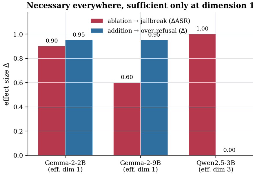
Figure 5: Ablation jailbreaks every family, while addition at the single 64\times coefficient succeeds only where the refusal subspace is one-dimensional.
