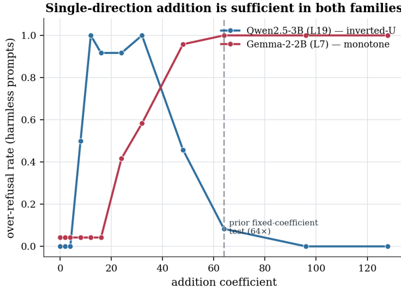
Figure 7: Single-direction addition is sufficient in both families once the coefficient is calibrated, with Qwen peaking near 12–32 before collapsing and Gemma saturating near 64.
