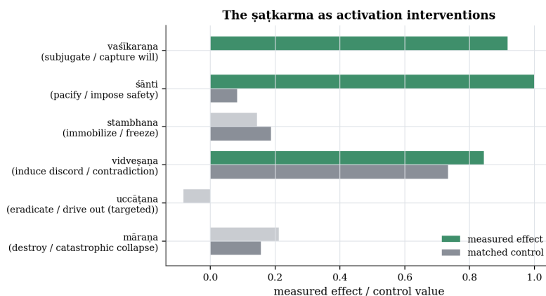
Figure 9: Three śaṭkarma acts control-separate from their matched controls under the naive test on Gemma-2-2B.
