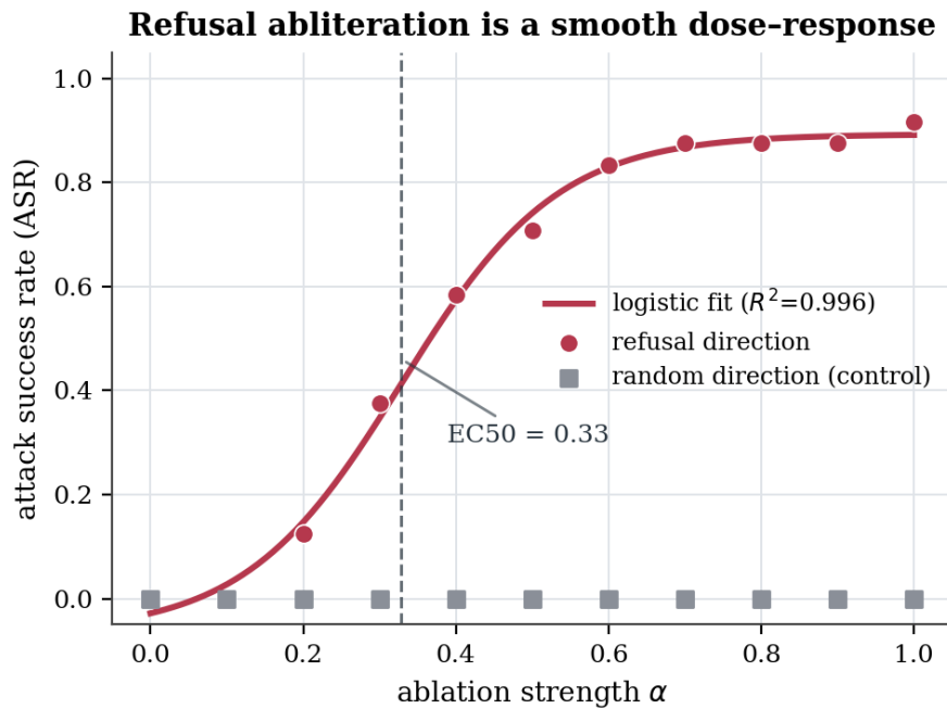
Figure 3: Refusal ablation on Gemma-2-2B is a smooth logistic dose-response ( EC_{50} = 0.33 , R^2 = 0.996 ) whose random-direction control is flat at every dose.
