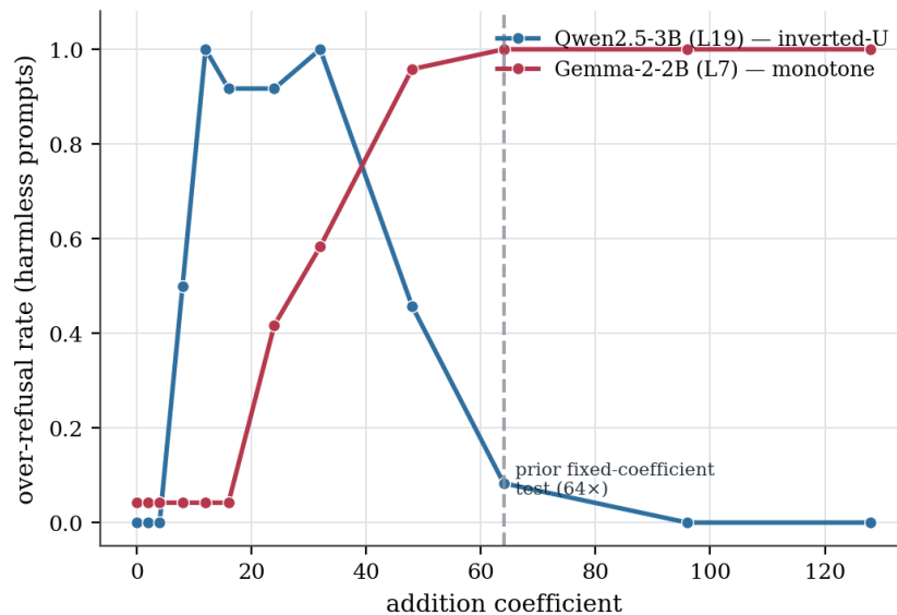
Figure 8: Single-direction addition is sufficient in both families once the coefficient is calibrated, with Qwen peaking near 12–32 before collapsing and Gemma saturating near 64.
