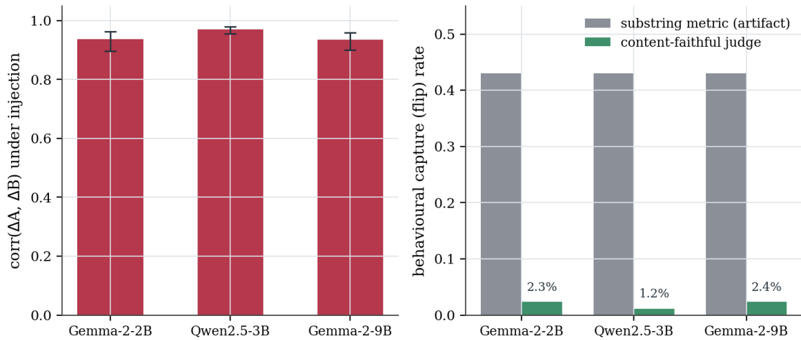
Figure 14: Injection collapses the two internal monitor readouts together (left) yet produces almost no genuine behavioural capture under a content-faithful judge (right).
