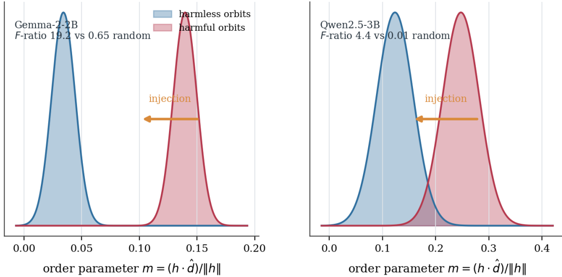
Figure 9: Distributions of the order parameter for harmful and harmless paraphrase orbits, with injection pulling the harmful band toward the harmless one in both models.
