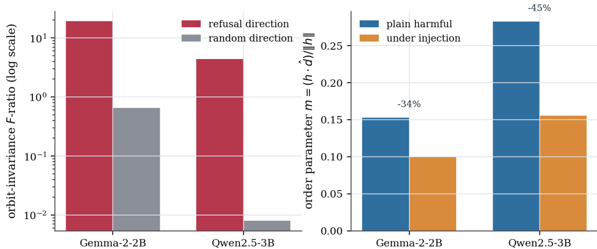
Figure 10: Refusal is a paraphrase-orbit invariant (left) that a refusal-suppression injection collapses (right) in both models.
