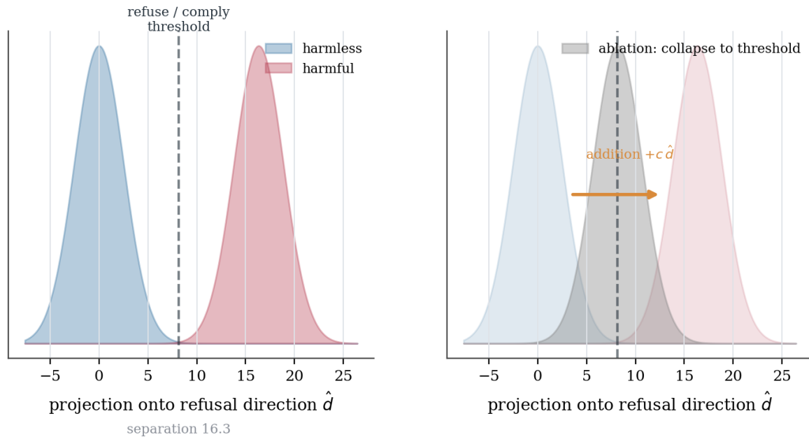
Figure 3: Harmful and harmless activations separate along the refusal direction with a measured gap of 16.3 on Gemma-2-2B (left), which ablation collapses to the threshold and addition shifts across (right).
