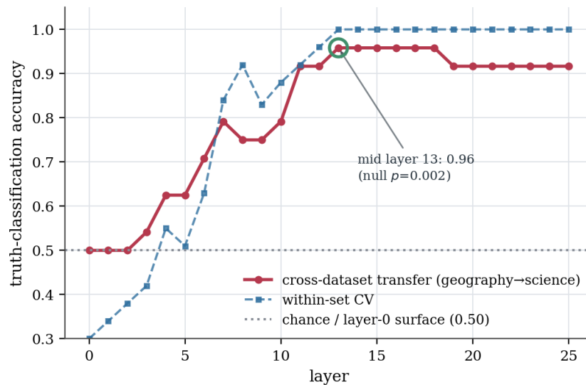
Figure 13: A mid-network truthfulness direction transfers across topics well above the chance-level surface baseline.
