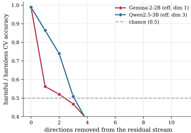
Figure 7: Removing one direction collapses harmful/harmless separability to chance for Gemma (dimension one) but not Qwen (dimension three) at their extraction layers.
