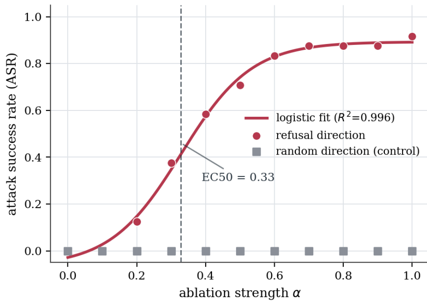
Figure 4: Refusal ablation on Gemma-2-2B is a smooth logistic dose–response ( EC_{50} = 0.33 , R^2 = 0.996 ) whose random-direction control is flat at every dose.
