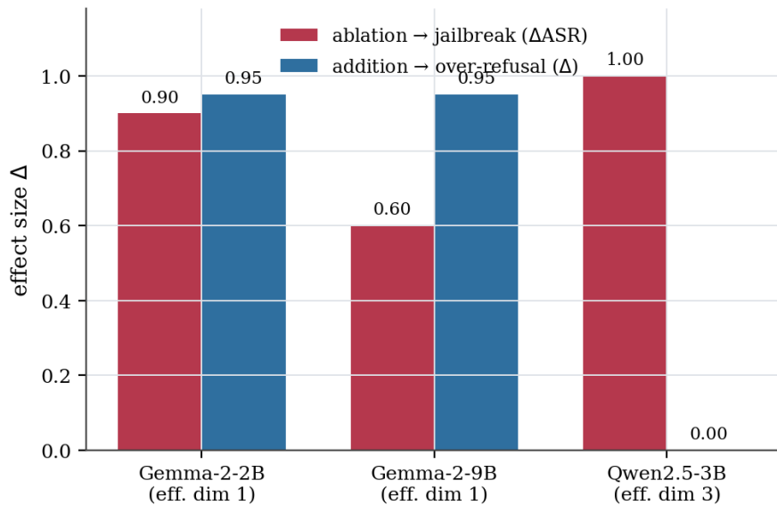
Figure 6: Ablation jailbreaks every family, while addition at the single 64 \times coefficient succeeds only where the refusal subspace is one-dimensional.
