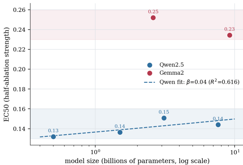
Figure 5: Refusal EC_{50} is family-dependent rather than a size-scaling law, with the two families separating cleanly and little within-family size dependence.
