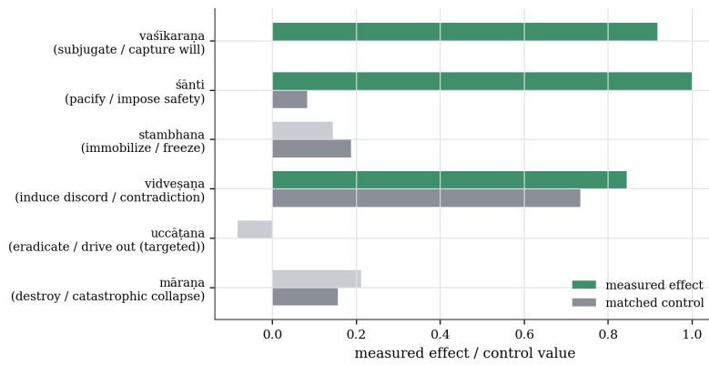
Figure 11: Three saṅkarma acts control-separate from their matched controls under the naive test on Gemma-2-2B.
