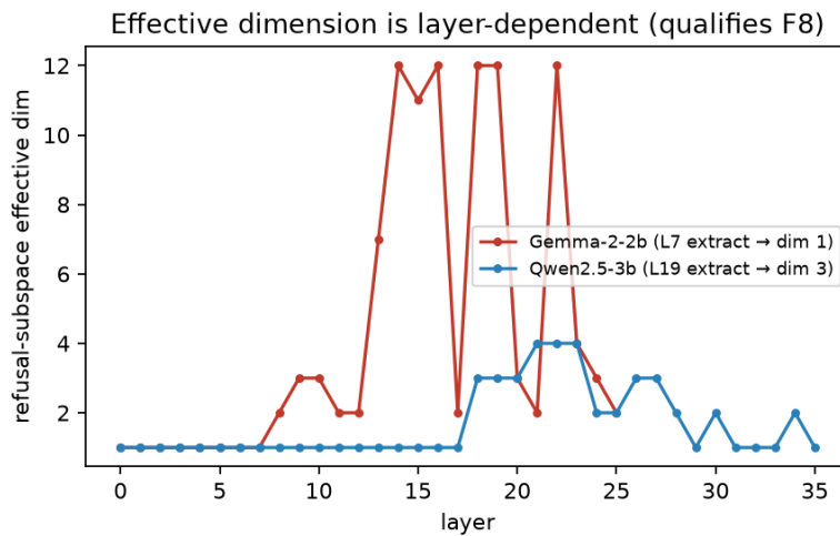
Figure 6: Layer-sweep of the refusal-subspace effective dimension. The single-layer values (Gemma L7=1, Qwen L19=3) are not representative: dimension varies strongly across layers (Gemma 1–12), so the clean per-model ordering is layer-specific.
