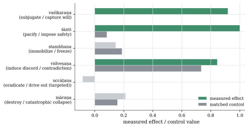
Figure 9: Three ṣaṭkarma acts control-separate from their matched controls under the naive test on Gemma-2-2B.
