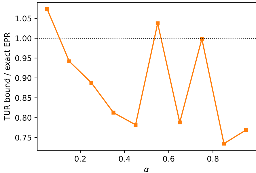
TUR tightness: saturation near equilibrium
