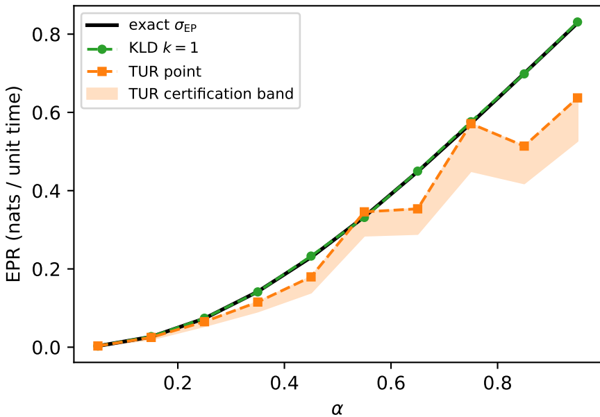
trajectory estimators vs exact
