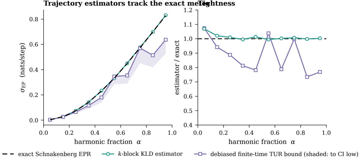
Figure 5. (a) Trajectory estimators against the exact entropy production. (b) Tightness. By construction the certified bound cannot exceed the exact value.
