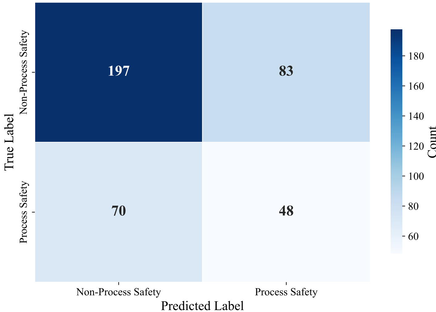
Confusion Matrix — NETHERLANDS_MANUAL (xlnet-base-cased)
