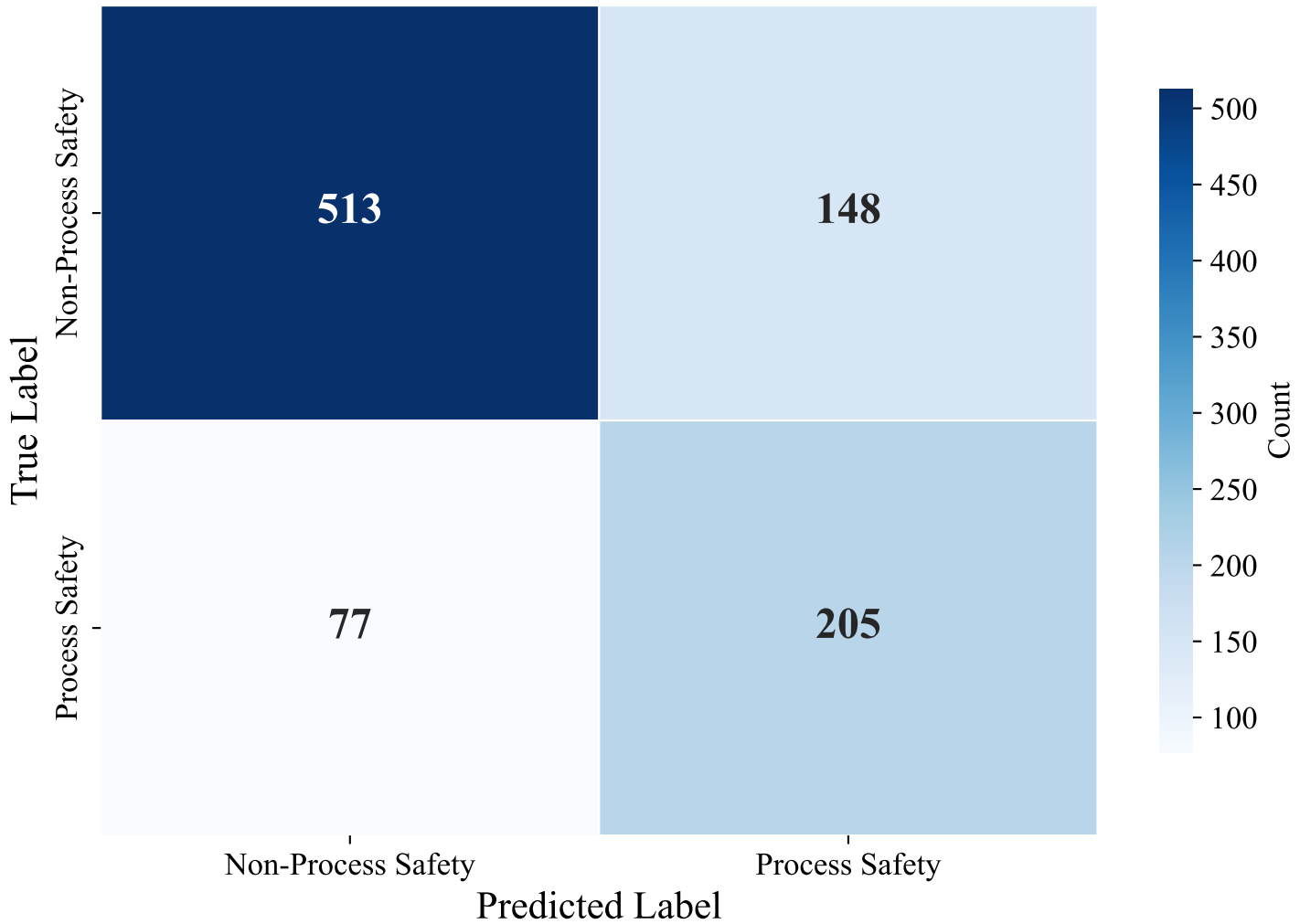
Confusion Matrix — ENGLISH_MANUAL (intfloat/multilingual-e5-base)
