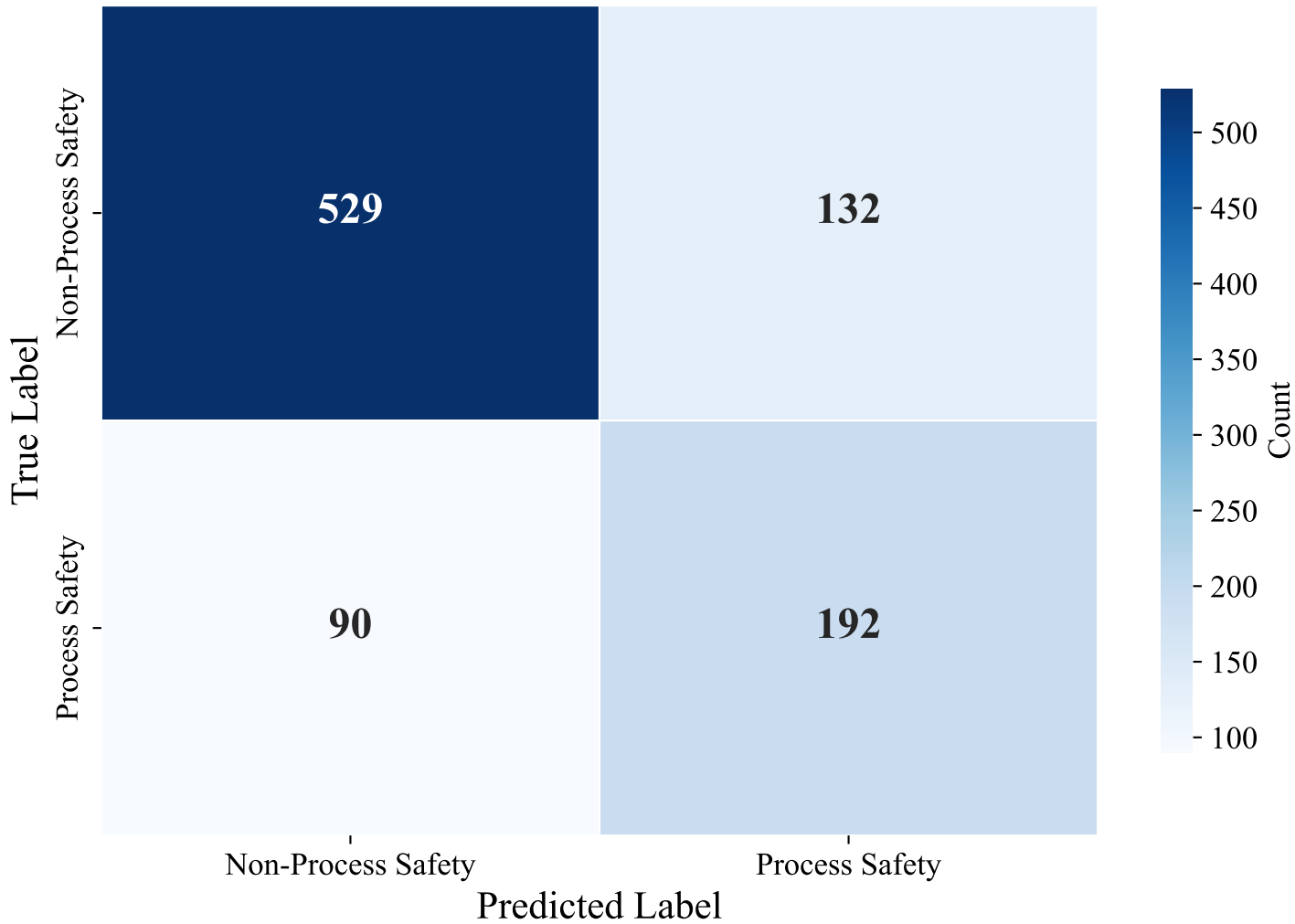
Confusion Matrix — ENGLISH_MANUAL (intfloat/multilingual-e5-large-instruct)
