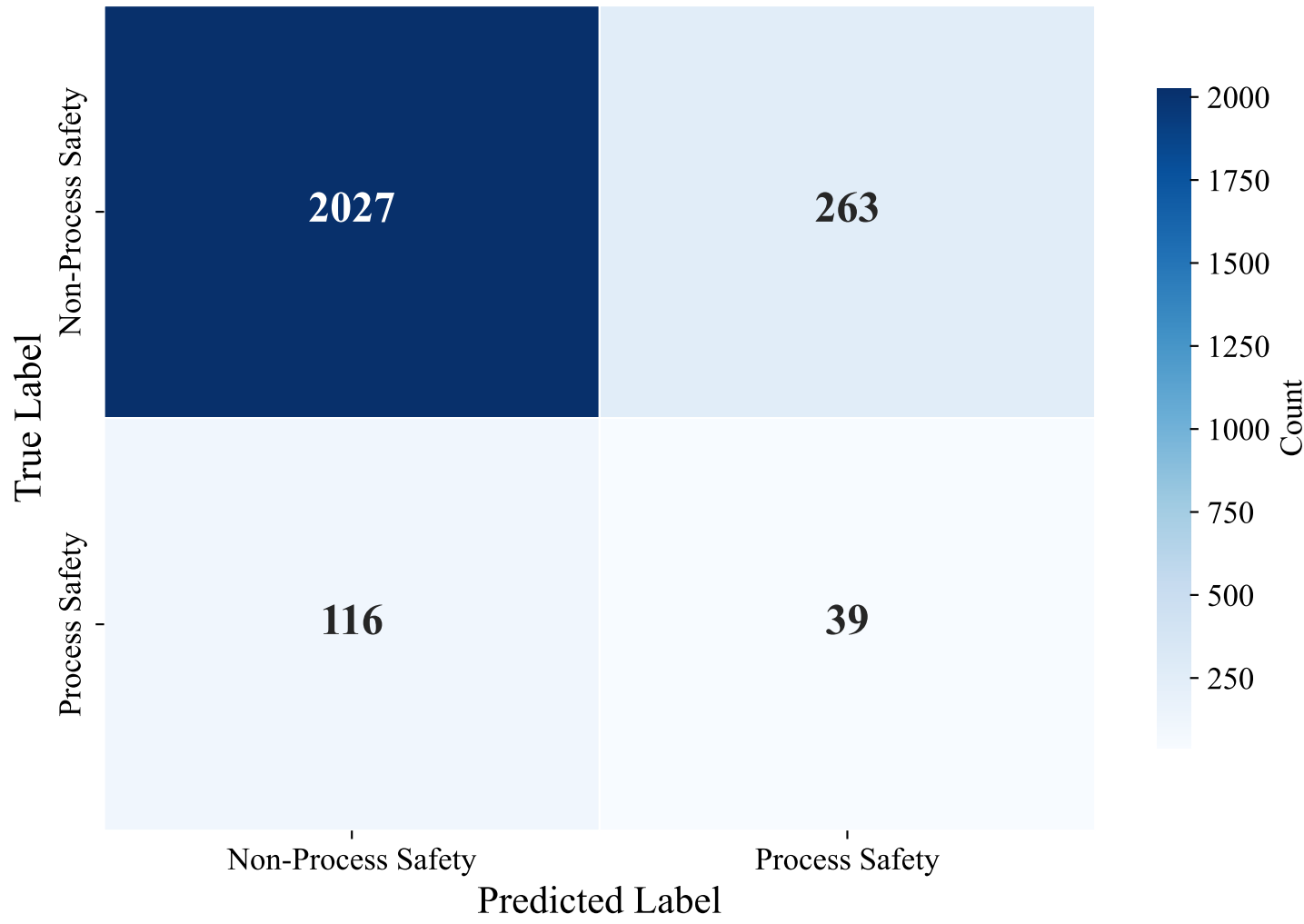
Confusion Matrix — SWEDEN_MANUAL (bert-base-multilingual-cased)
