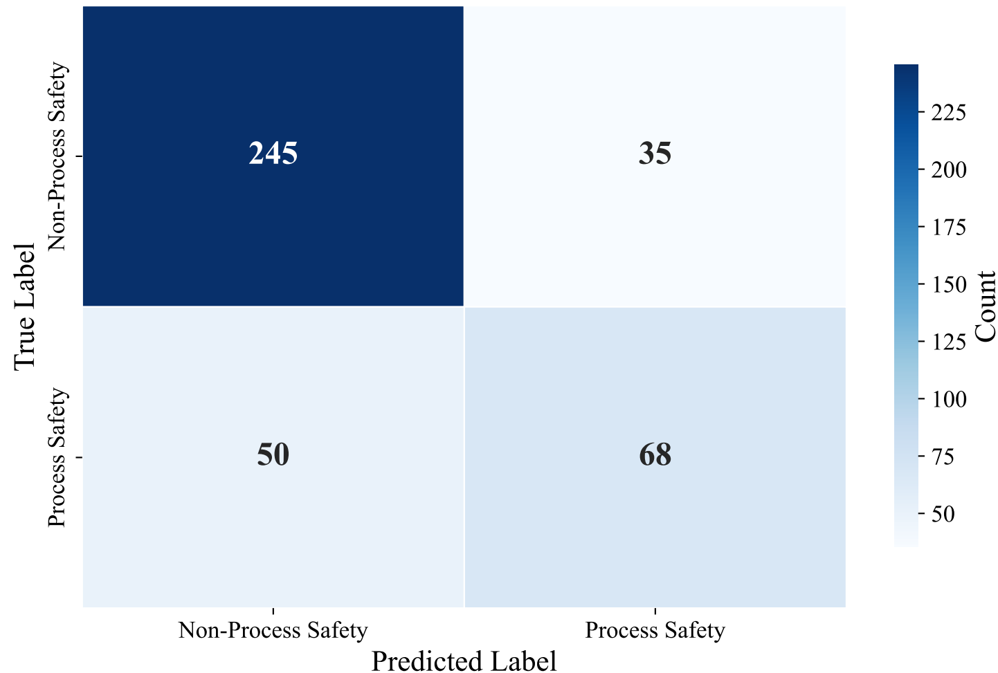
Confusion Matrix — DUTCH_MANUAL (Alibaba-NLP/gte-multilingual-base, LightGBM)
