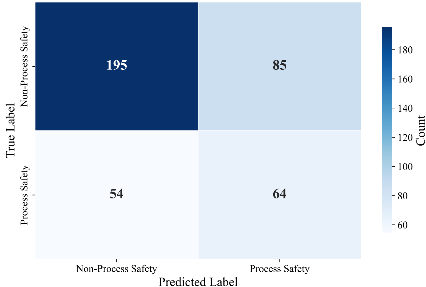
Confusion Matrix — DUTCH_MANUAL (Alibaba-NLP/gte-multilingual-base, SVM)
