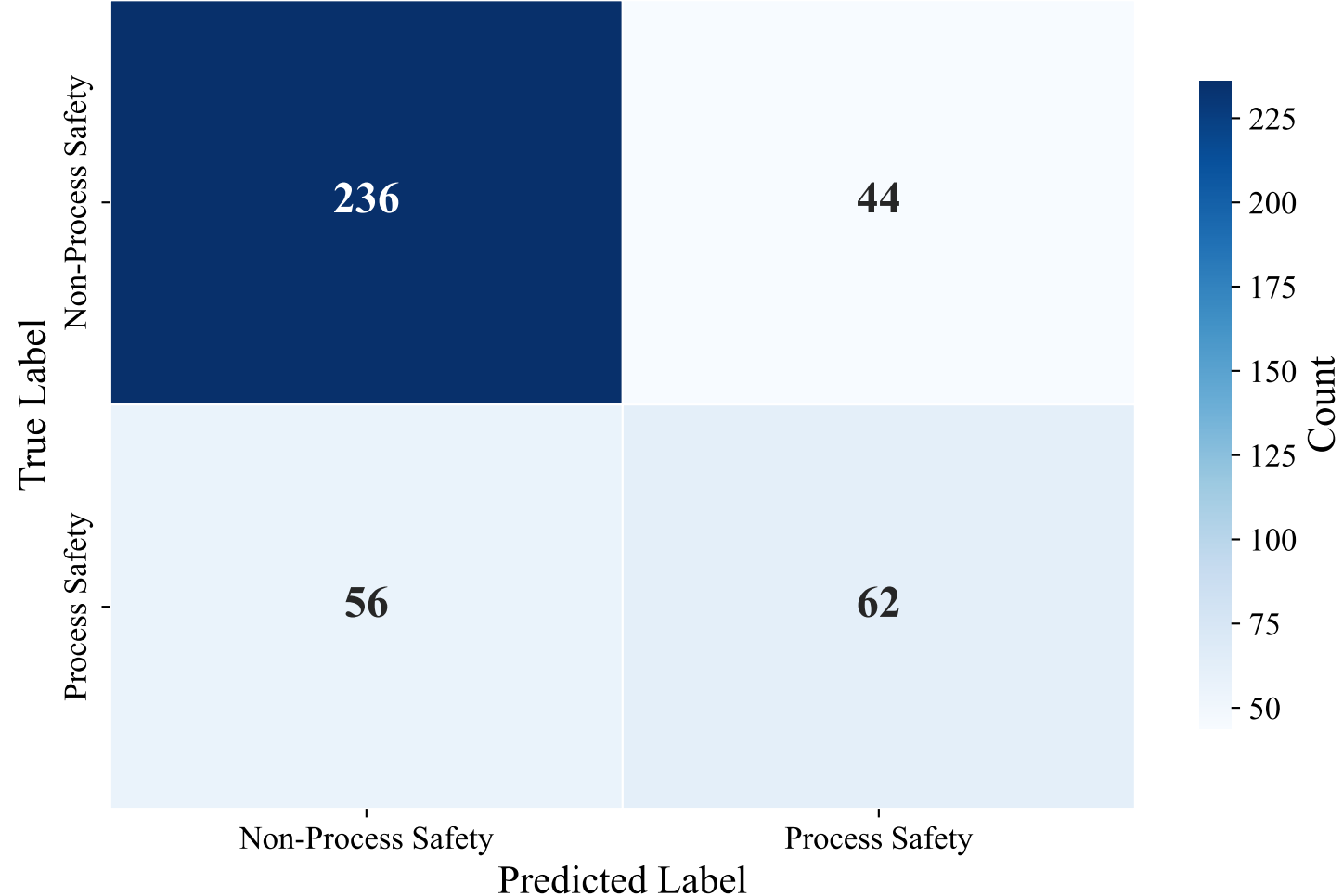
Confusion Matrix — DUTCH_MANUAL (bert-base-multilingual-uncased, LightGBM)
