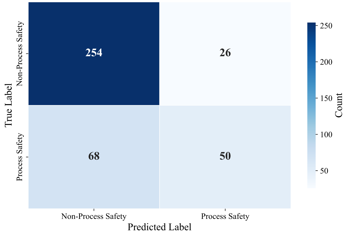
Confusion Matrix — DUTCH_MANUAL (intfloat/multilingual-e5-large-instruct, Random_Forest)
