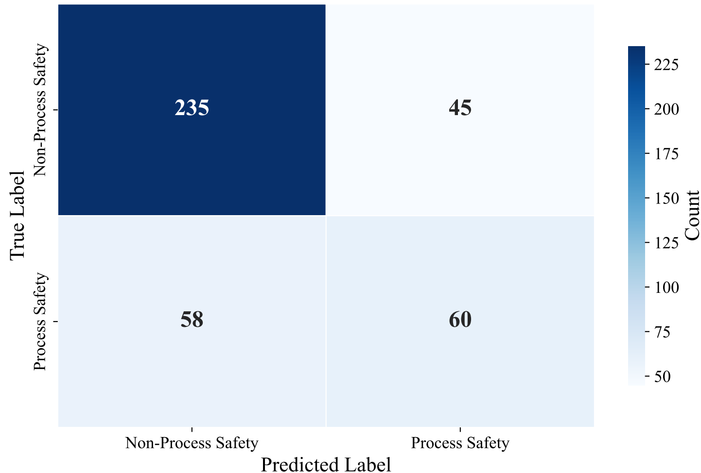
Confusion Matrix — DUTCH_MANUAL (paraphrase-multilingual-MiniLM-L12-v2, Voting_Ensemble)
