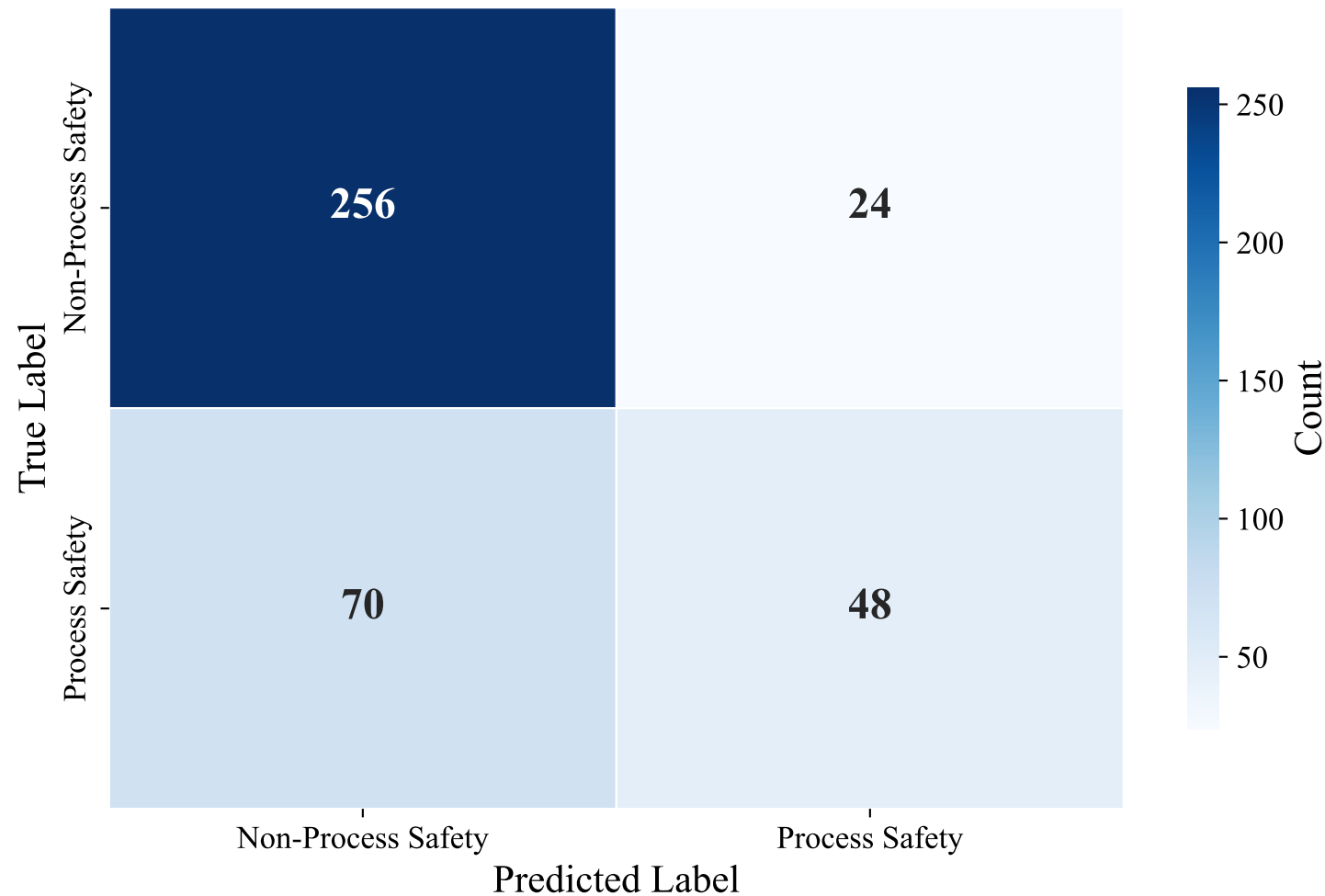
Confusion Matrix — DUTCH_MANUAL (paraphrase-multilingual-mpnet-base-v2, Random_Forest)
