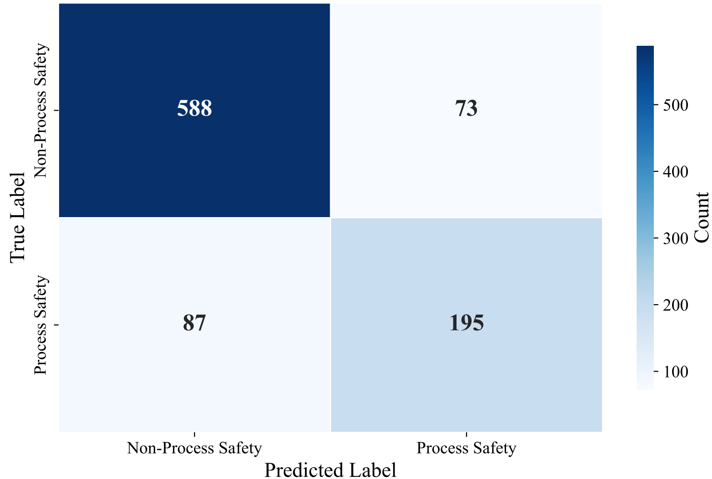
Confusion Matrix — ENGLISH_MANUAL (intfloat/multilingual-e5-large-instruct, LightGBM)
