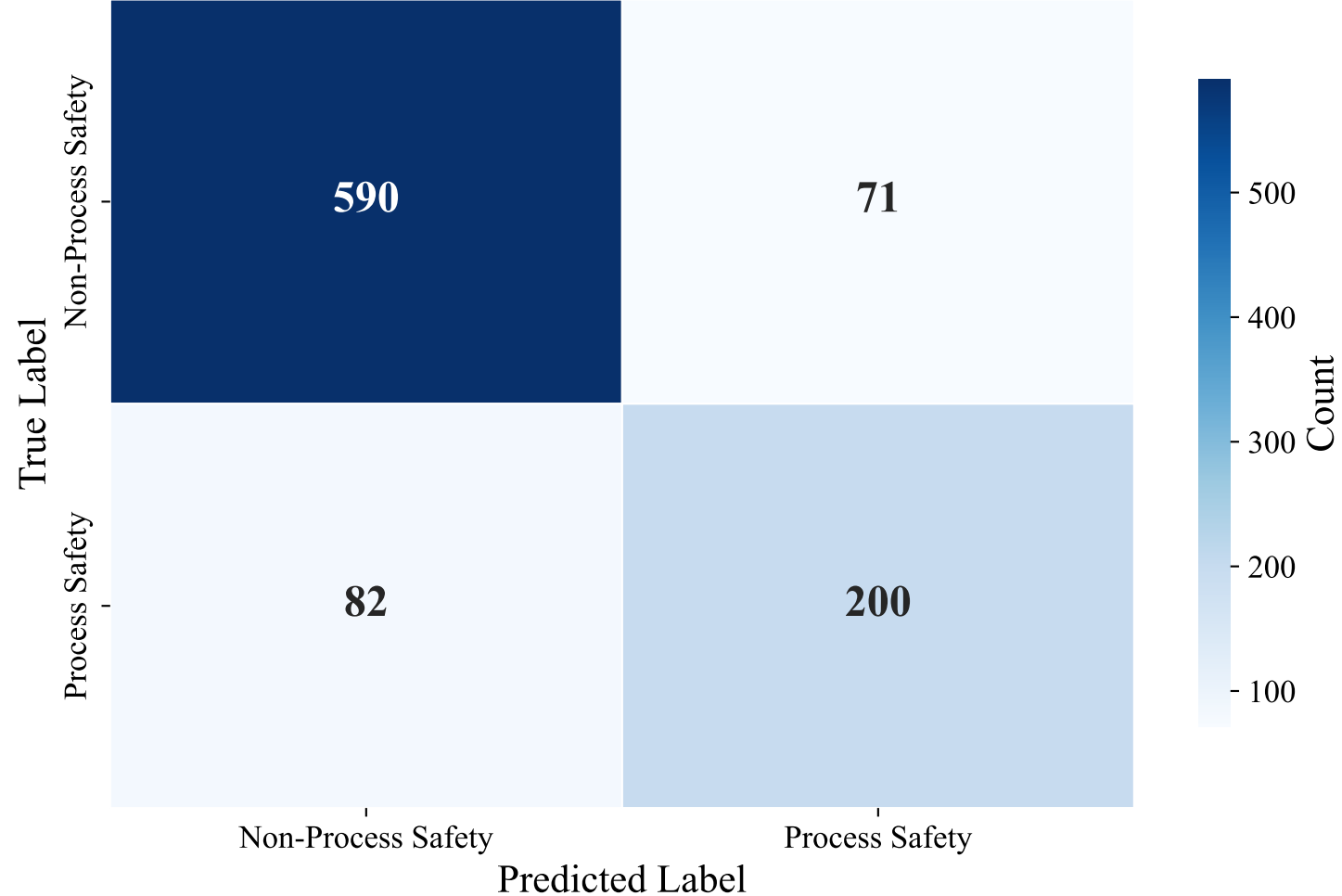
Confusion Matrix — ENGLISH_MANUAL (snowflake-arctic-embed-l-v2.0, XGBoost)
