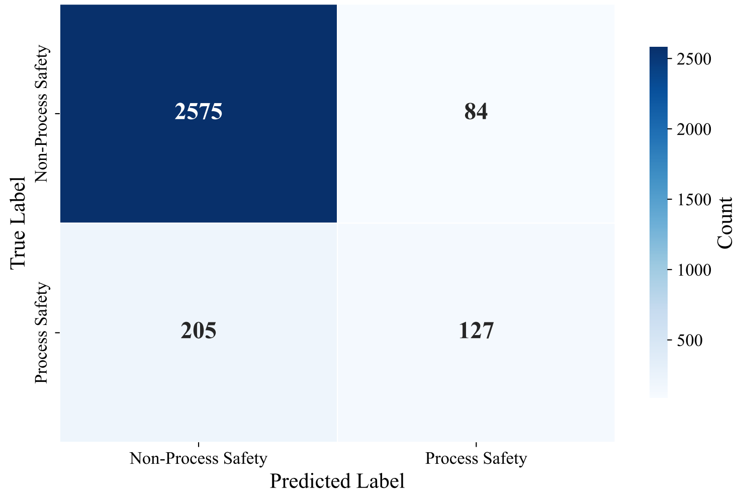
Confusion Matrix — GERMAN_MANUAL (Alibaba-NLP/gte-multilingual-base, Random_Forest)
