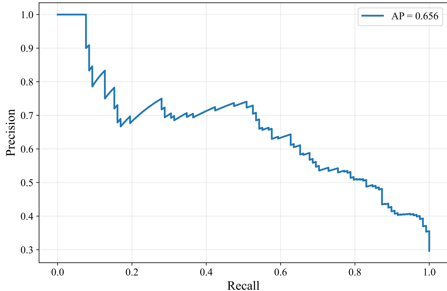
Precision-Recall Curve — DUTCH_MANUAL (Alibaba-NLP/gte-multilingual-base, LightGBM)
