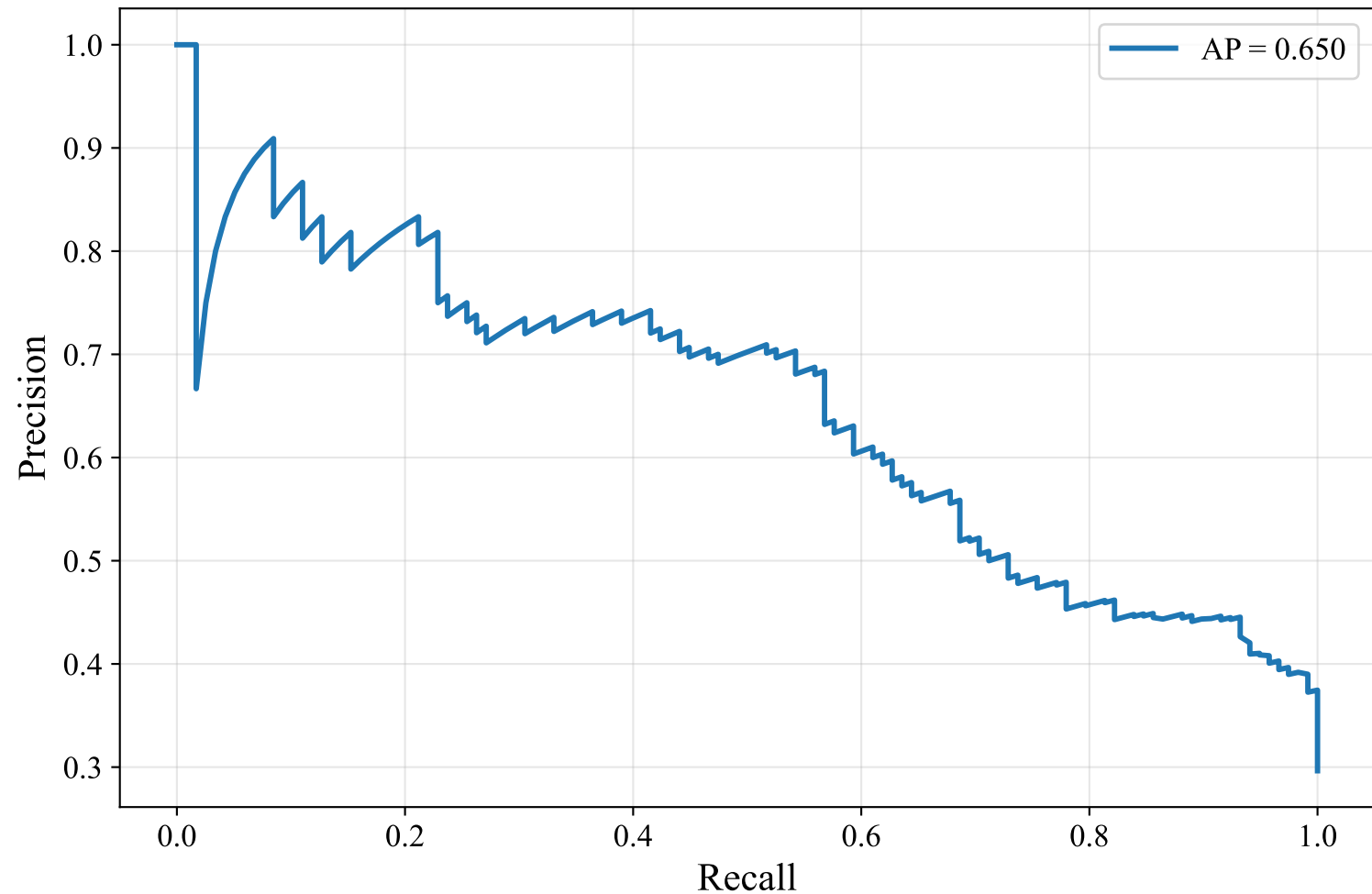
Precision-Recall Curve — DUTCH_MANUAL (Alibaba-NLP/gte-multilingual-base, Random_Forest)
