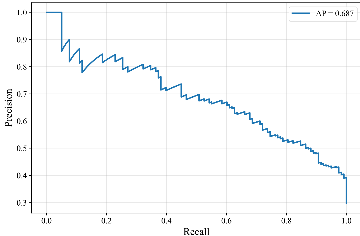
Precision-Recall Curve — DUTCH_MANUAL (intfloat/multilingual-e5-large-instruct, LightGBM)
