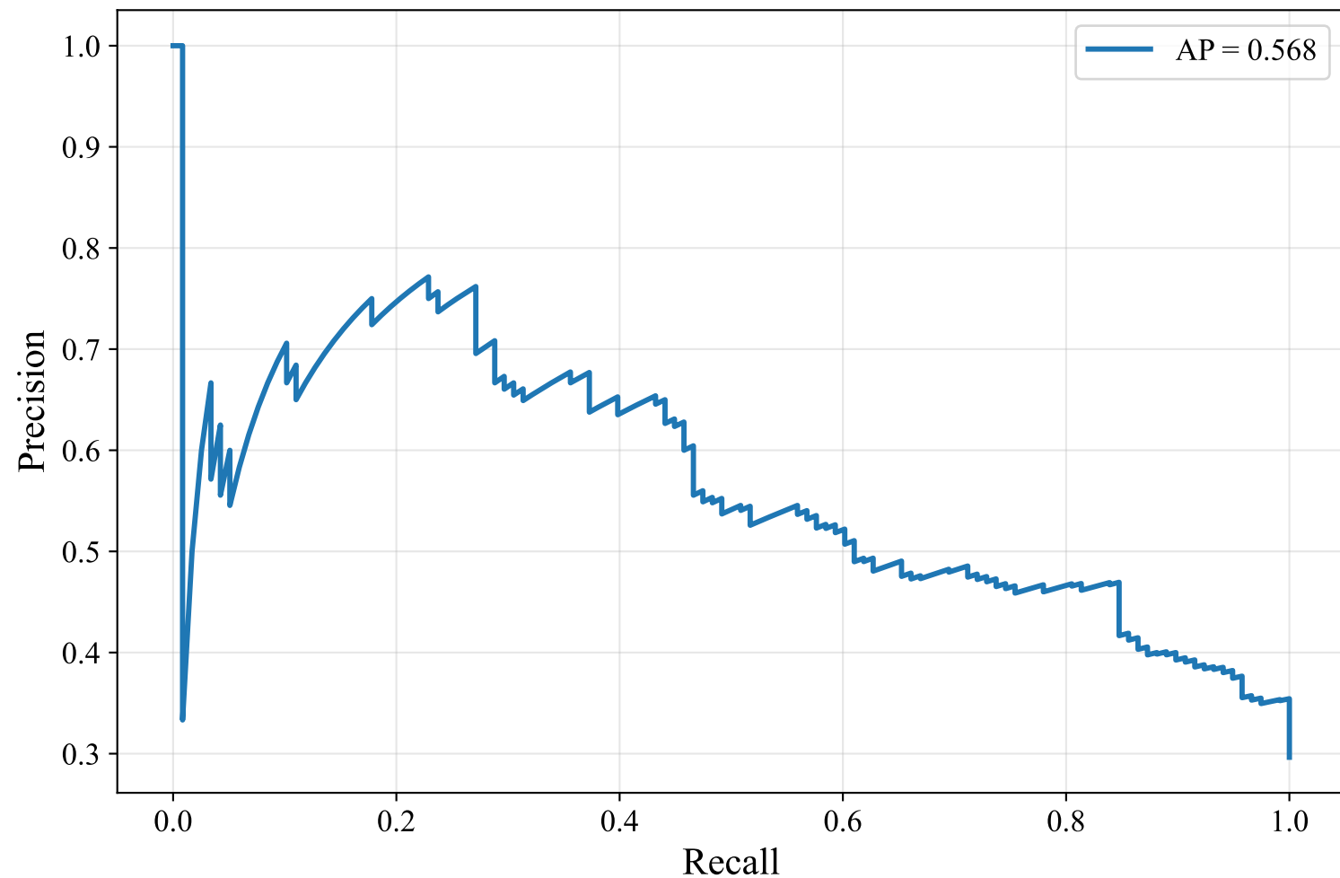
Precision-Recall Curve — DUTCH_MANUAL (paraphrase-multilingual-MiniLM-L12-v2, LightGBM)
