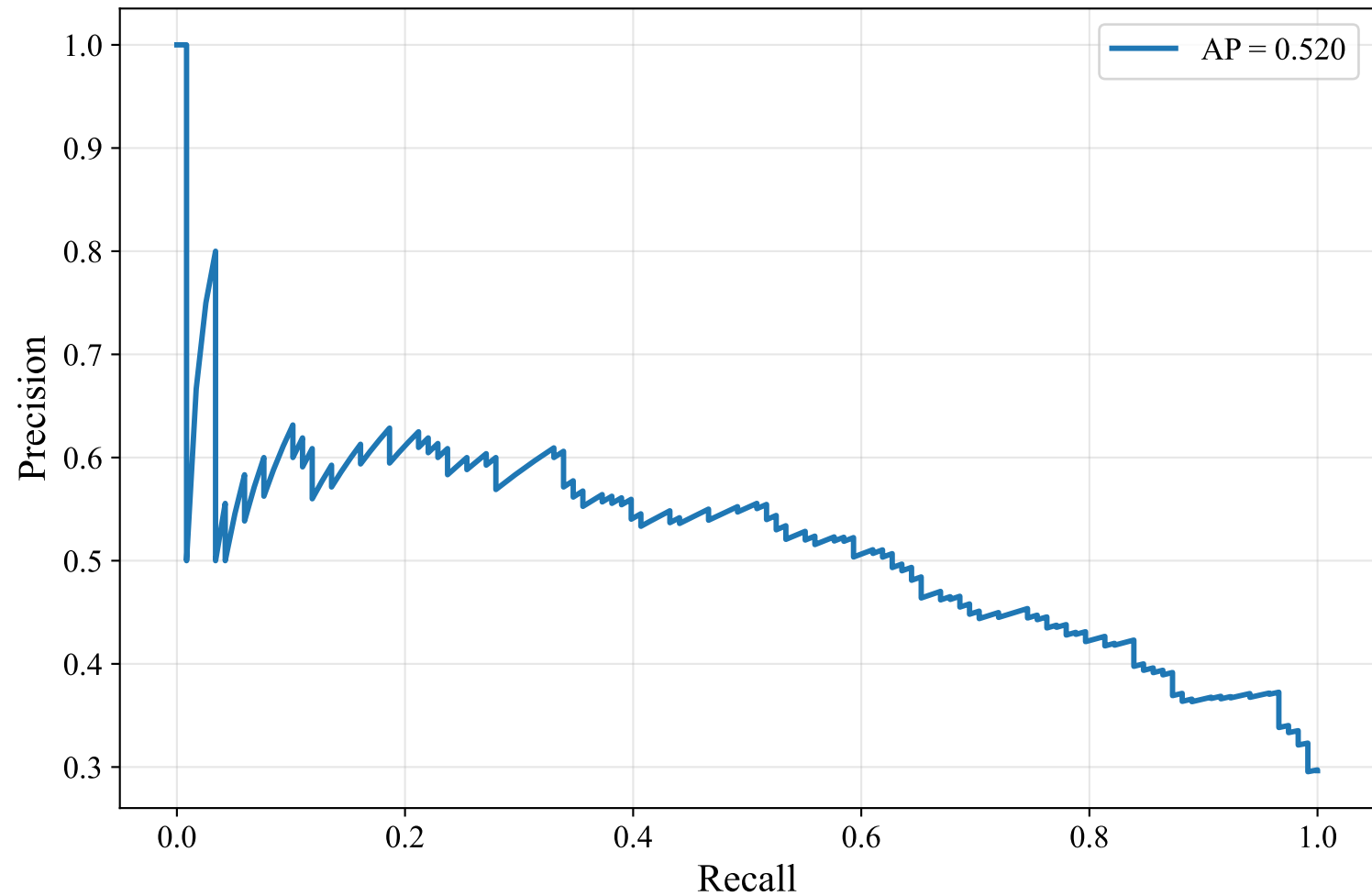
Precision-Recall Curve — DUTCH_MANUAL (paraphrase-multilingual-MiniLM-L12-v2, SVM)
