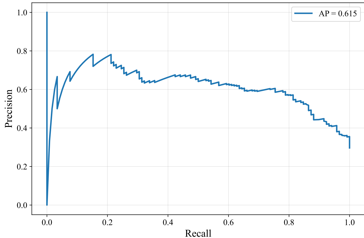
Precision-Recall Curve — DUTCH_MANUAL (paraphrase-multilingual-mpnet-base-v2, Random_Forest)
