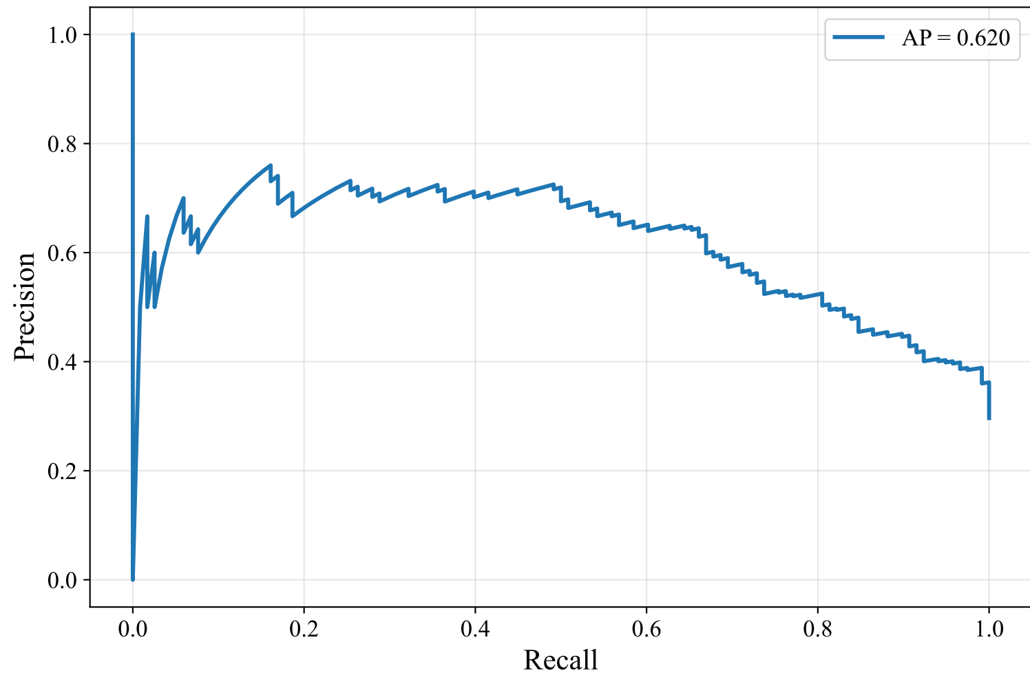
Precision-Recall Curve — DUTCH_MANUAL (xlm-roberta-base, XGBoost)
