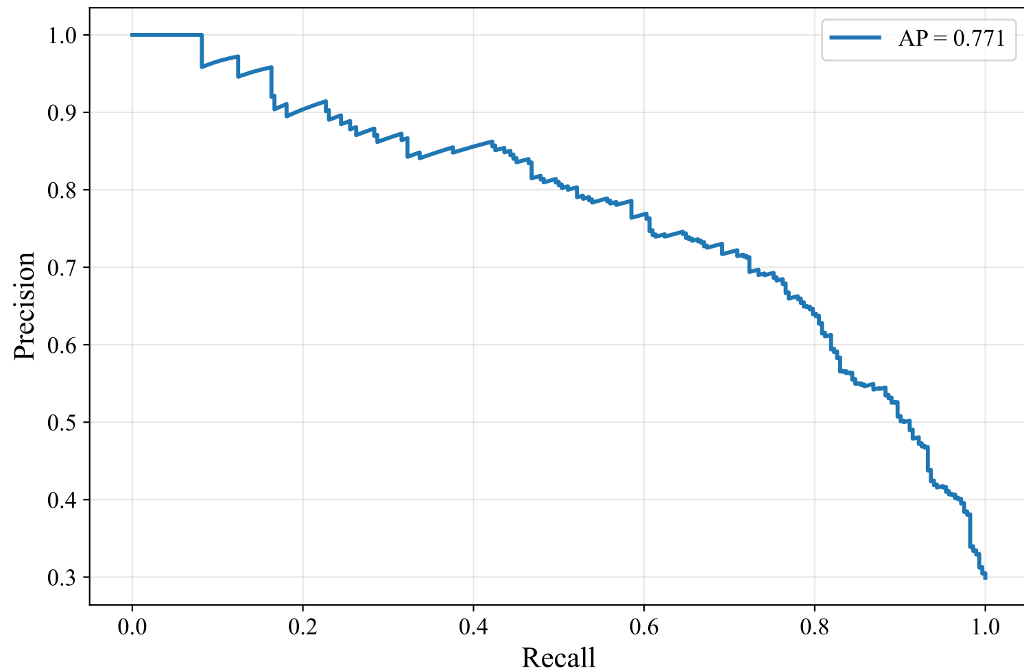
Precision-Recall Curve — ENGLISH_MANUAL (intfloat/multilingual-e5-large-instruct, LightGBM)
