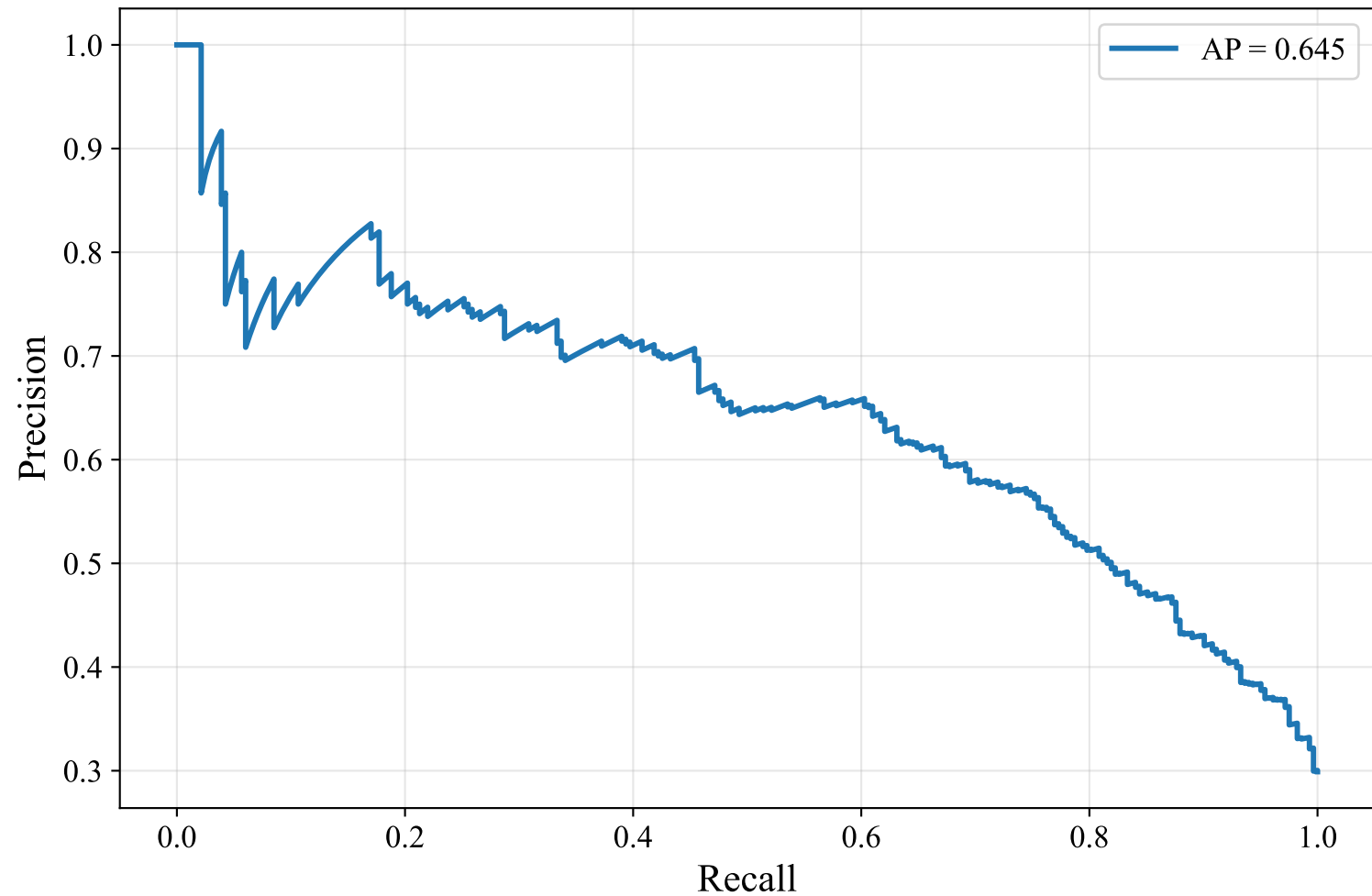
Precision-Recall Curve — ENGLISH_MANUAL (intfloat/multilingual-e5-large-instruct, SVM)
